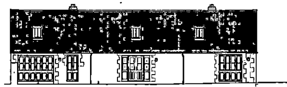
EAST ELEVATION AS EXISTING
