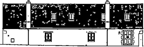
WEST ELEVATION AS EXISTING SCALE 1:100
