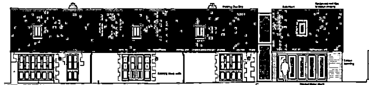
EAST ELEVATION AS PROPOSED SCALE 1:100
